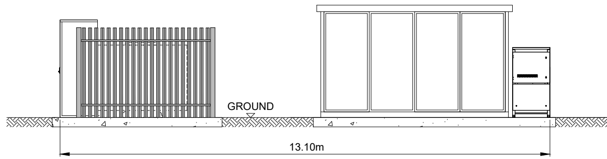
ELEVATION 'A'
