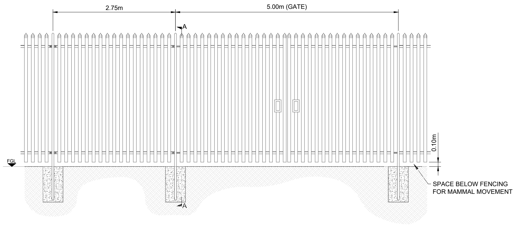
TYPICAL PALISADE FENCE DETAIL
